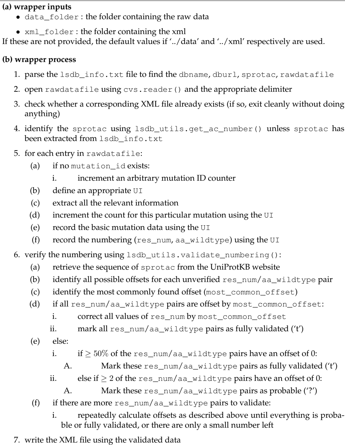
Figure 3.4: The PD data wrapper: pseudocode
