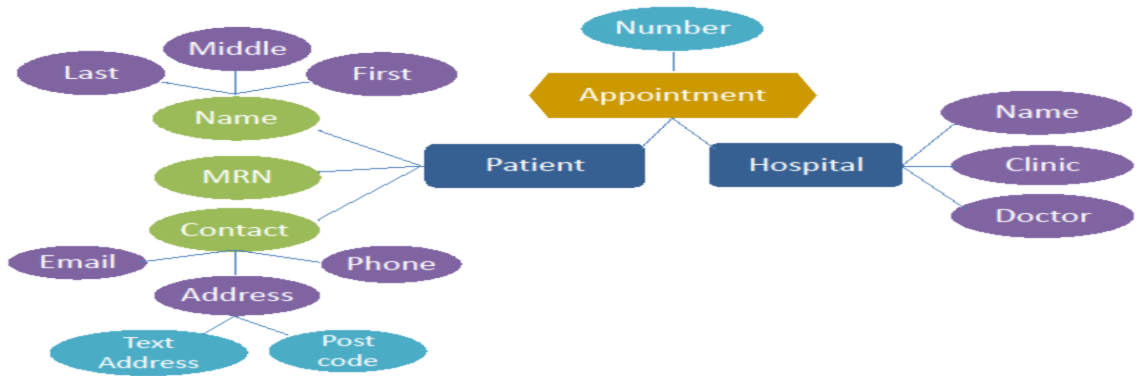
(a) An example entity relationship (ER) diagram. Entities are in square-edged rectangles while attributes are in oval boxes; lines join entities and relationships to their attributes.
