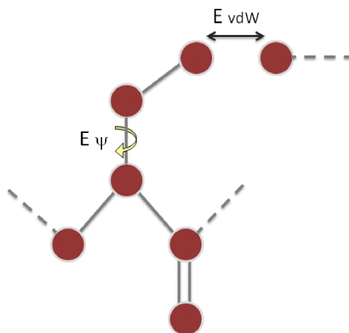
Figure 4.6: Schematic indicating the two new terms used in evaluation of clashes. E_{vdW} is the van der Waals energy evaluated using a standard Lennard-Jones potential while E_{\psi} is the torsion energy.
