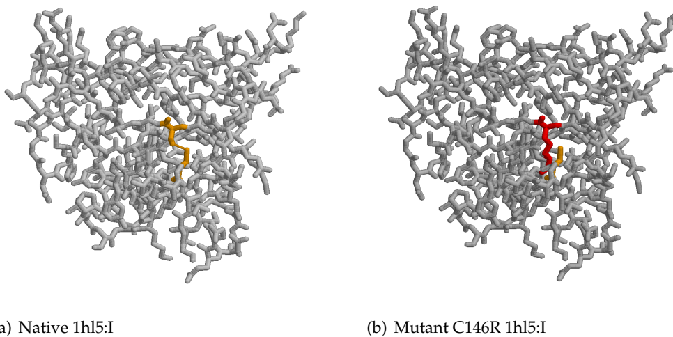
Figure 3.13: Disrupting disulphide bonding.
