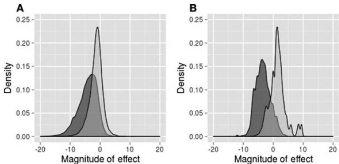
Figure 2.12: Disease-associated (shaded region) and functionally neutral (un-shaded region) amino acid substitutions in the SwissVar dataset using un-weighted and weighted methods (A and B, respectively). A prediction thresholds were calculated at which both specificity and sensitivity were maximized (-3.0 and -1.5, respectively) (Shihab et al. , 2013).
