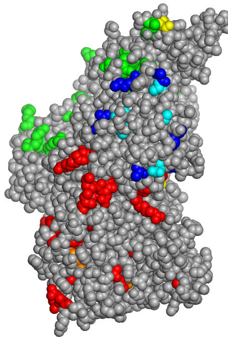
Figure 7.4: Clustering MYHC mutation on PDB ID 4db1 human myosin structure. Colouring the clusters red, green and blue for HCM and orange, yellow and cyan for DCM.
