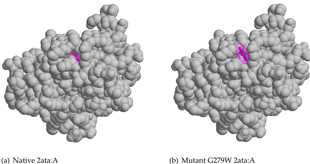
Figure 3.9: Residues found to clash with other existing residues.
