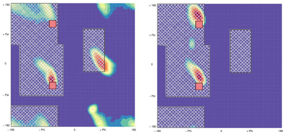
(a) Glycine - The allowed regions for glycine using the previous method where non -pink area marks the conformational space, primarily occupied by glycine residues.
