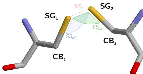
Figure 3.12: A disulphide bond between C6 and C127 of lysozyme (7lyz), showing SS_d , SS_{a1} and SS_{a2}
