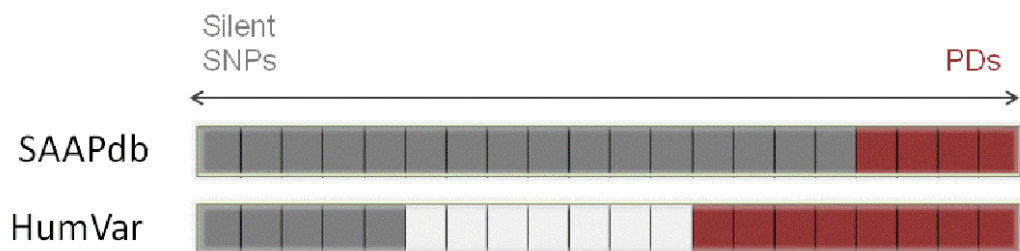
Figure 6.7: The penetrance of a mutation lies on a scale between ‘True SNPs’ which show no phenotypic effect at one extreme to Mendelianly inherited PDs with 100% penetrance at the other. In SAAPdb, we use a very conservative definition of PDs, but a rather wide definition of SNPs. In contrast, HumVar uses a somewhat broader definition of PDs, but a much more conservative definition of SNPs and does not consider mutations that lie in the middle.
