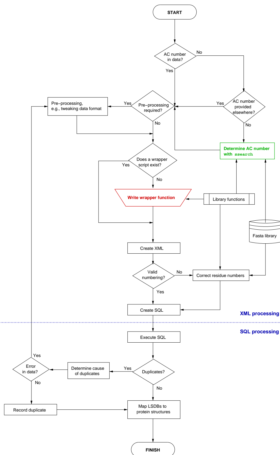
Figure 3.3: Importing an LSMDB dataset.
