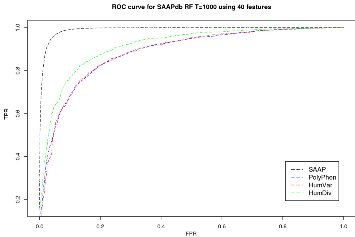
Figure 6.5: ROC curves of SAAPpred predictor training on different dataset SAAPdb, Polyphen (HumVar + HumDir), HumVar and HumDiv dataset. Results from WEKA 10-fold cross-validation.
