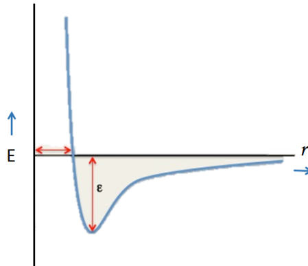
Figure 1.11: Lennard-Jones potential.
