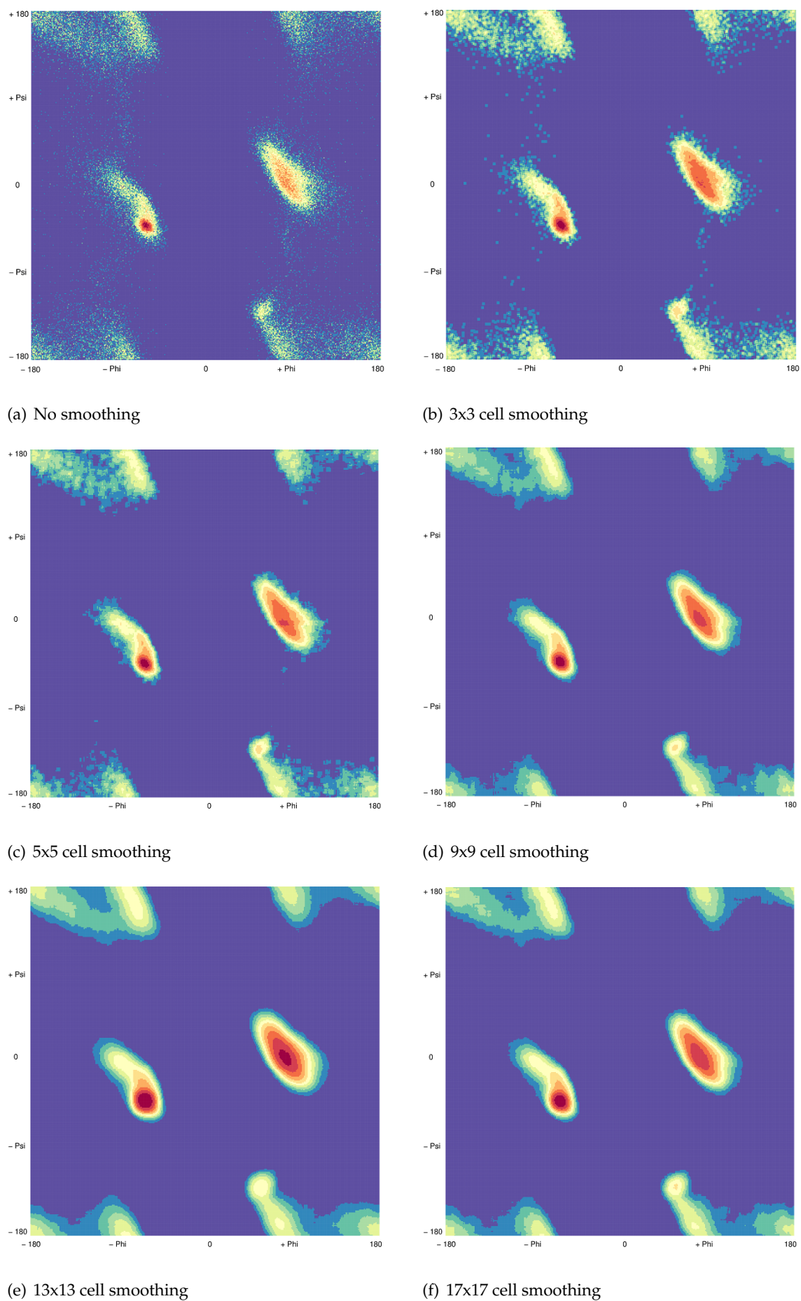
Figure 5.9: Glycine TDM smoothing.
