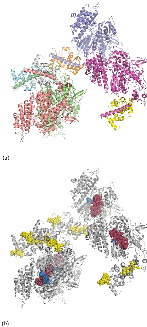
Figure 7.1: Cardiac human myosin S1dC, beta isoform complexed with Mn-AMPPNP PDB ID 1br4. (a) The structure of 1br4 showing the 8 chains in different colours. (b) actin-binding site (residues 655-677) coloured in ruby; the ATP-binding region (residues 178-185) coloured in blue; myosin light chain binding regions (residues 788-801 and 814-827) coloured in yellow.
